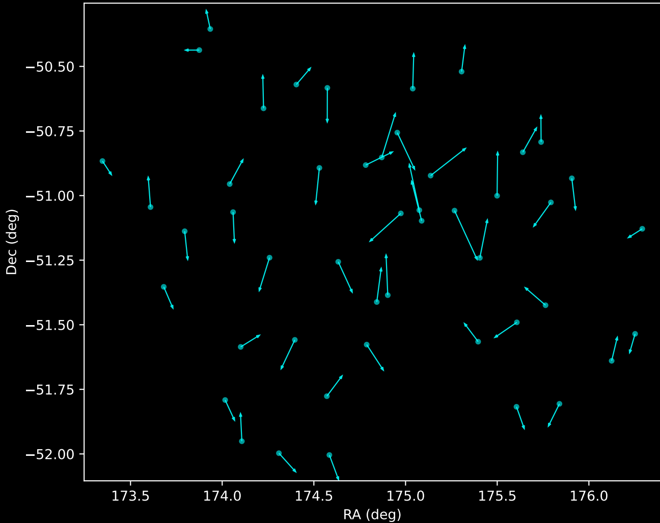
GALAH DR4 Noise Stream Proper Motion Vectors (n=48)
