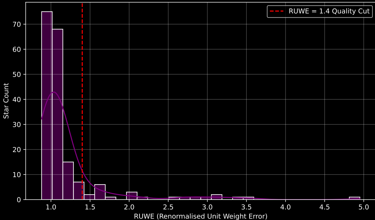
GALAH DR4 Field [338] RUWE Distribution (n= 187)
