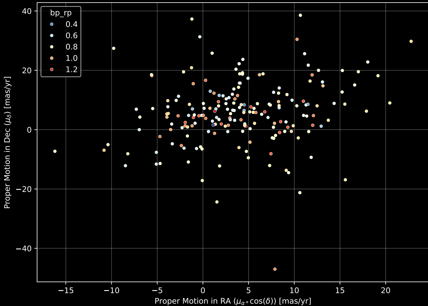
GALAH DR4 Field: [338] Proper Motion Diagram (n= 196)
