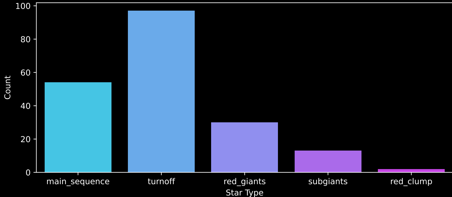
GALAH DR4 Field: [338] Count plot of Star Type
